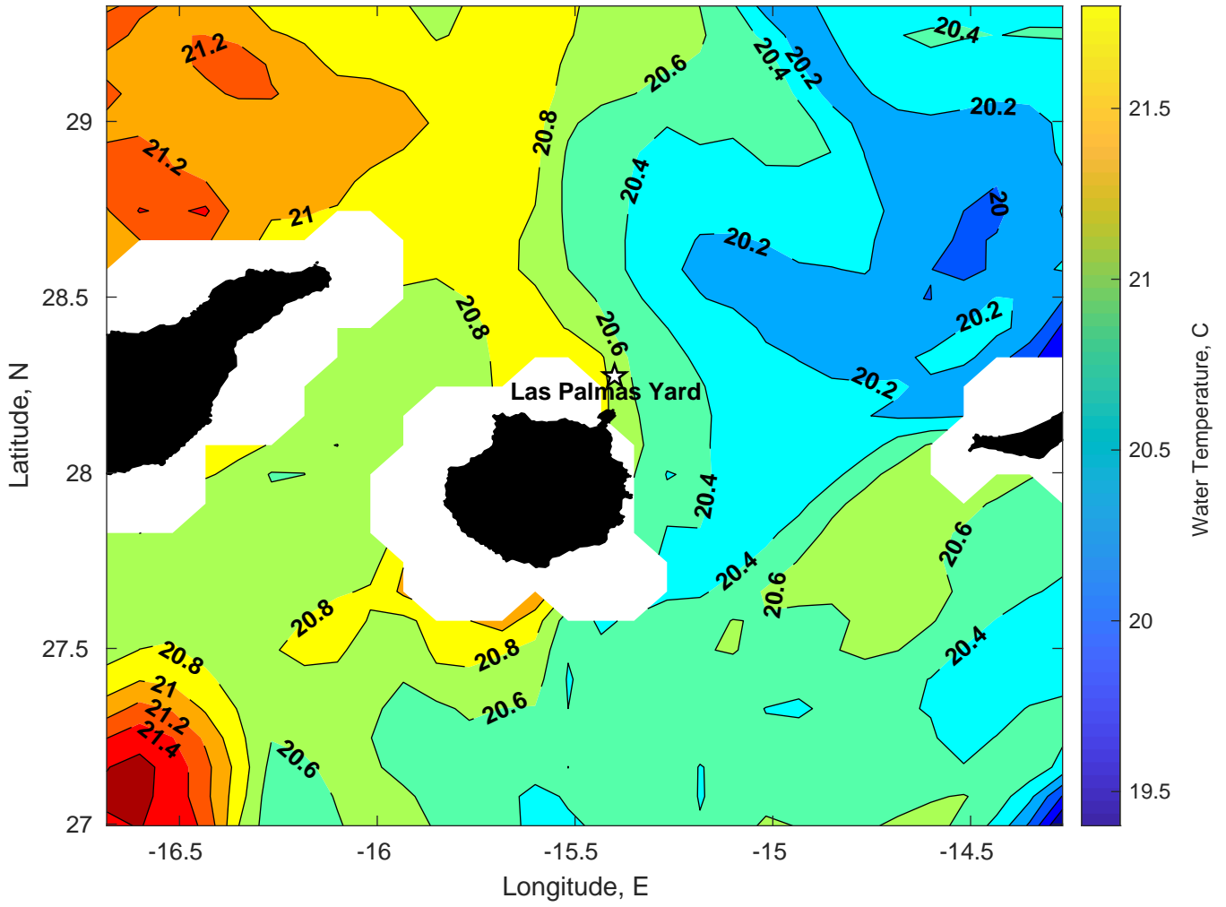
SST for Las Palmas Yard at 04-May-2024 00:00:00
